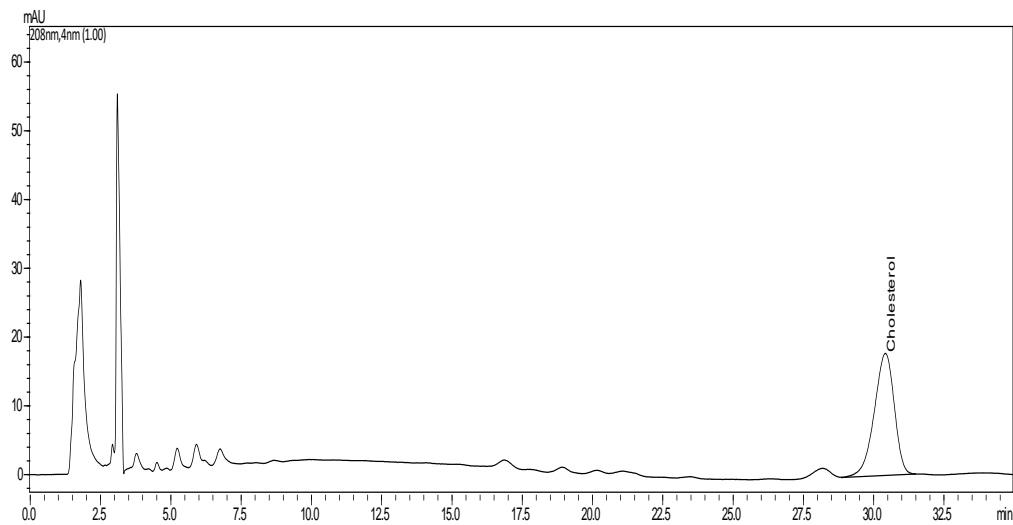
Figure 1. A sample HPLC-PDA chromatogram corresponding to the analysis of egg yolk cholesterol at 208 nm.
