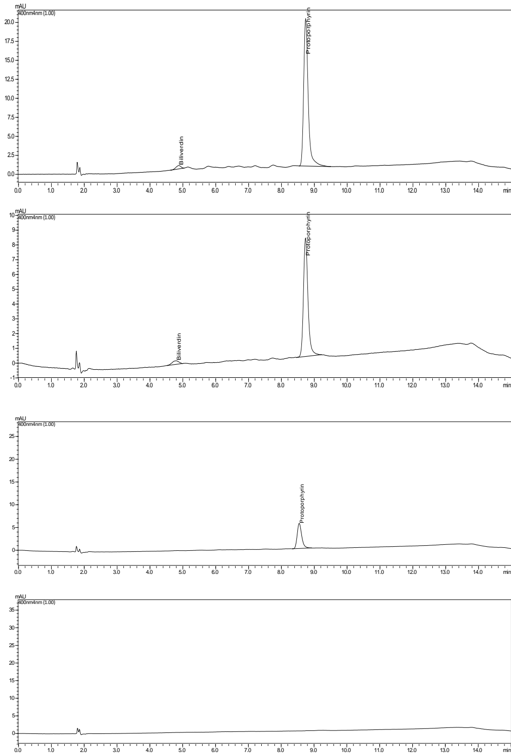
Figure 3. A sample HPLC-PDA chromatogram is corresponding to the analysis of protoporphyrin in quail eggshell (a), pheasant eggshell (b), chicken (organic) eggshell (c) and goose eggshell (d) at 400 nm.
